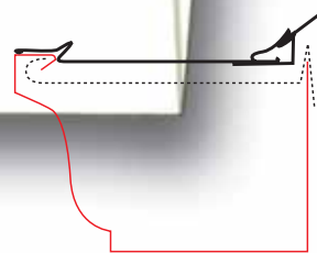
M-5100 Series Installation on hidden hangers or spikes and ferules
