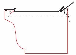
M-5300 Series Installation on hidden hangers or spikes and ferules
